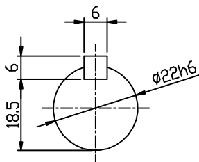
OUTPUT SHAFT
