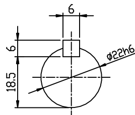
OUTPUT SHAFT
