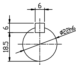
OUTPUT SHAFT
