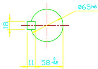
OUTPUT SHAFT
