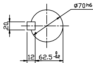
OUTPUT SHAFT
