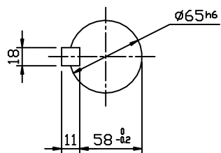
OUTPUT SHAFT
