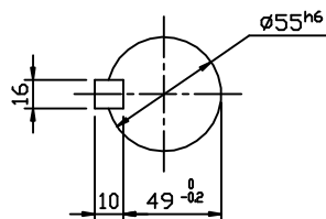
OUTPUT SHAFT
