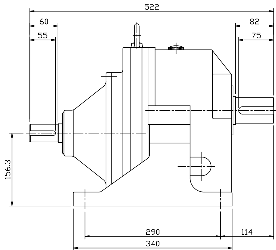
OUTPUT SHAFT
