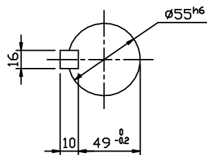
OUTPUT SHAFT
