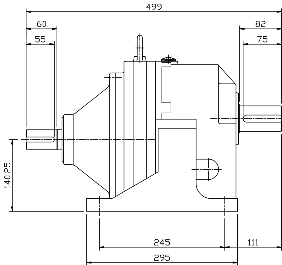
OUTPUT SHAFT
