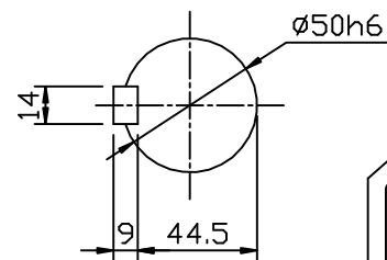
OUTPUT SHAFT
