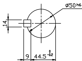
OUTPUT SHAFT
