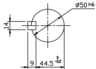
OUTPUT SHAFT
