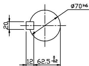
OUTPUT SHAFT
