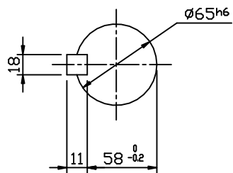
OUTPUT SHAFT
