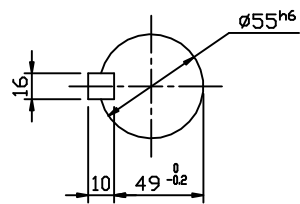
OUTPUT SHAFT
