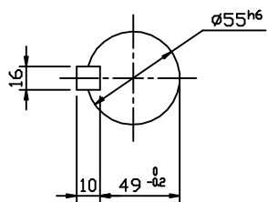
OUTPUT SHAFT
