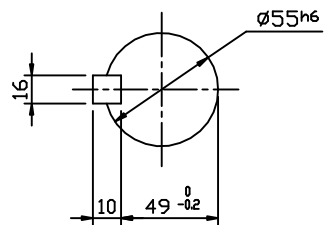
OUTPUT SHAFT
