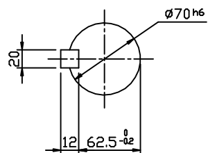
OUTPUT SHAFT
