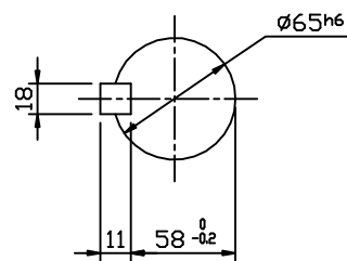
OUTPUT SHAFT
