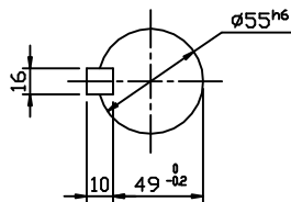
OUTPUT SHAFT
