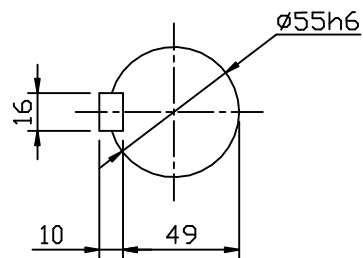
OUTPUT SHAFT
