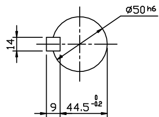
OUTPUT SHAFT
