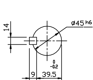
OUTPUT SHAFT
