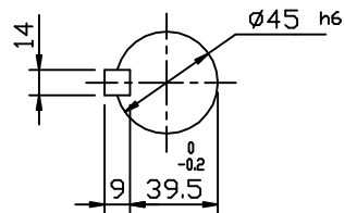
OUTPUT SHAFT
