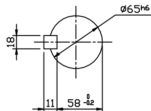
OUTPUT SHAFT
