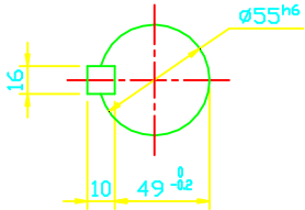
OUTPUT SHAFT
