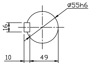
OUTPUT SHAFT
