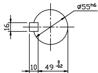
OUTPUT SHAFT
