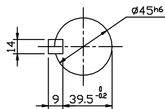
OUTPUT SHAFT
