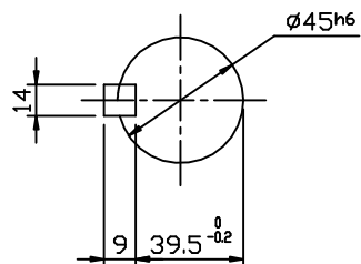
OUTPUT SHAFT
