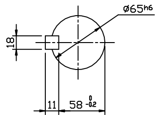
OUTPUT SHAFT
