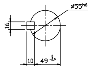
OUTPUT SHAFT
