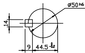
OUTPUT SHAFT
