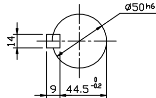
OUTPUT SHAFT
