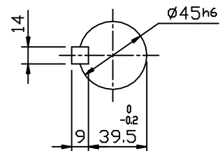
OUTPUT SHAFT
