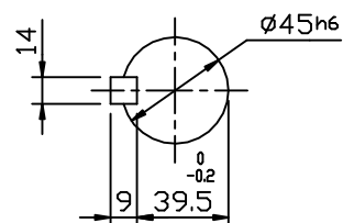
OUTPUT SHAFT
