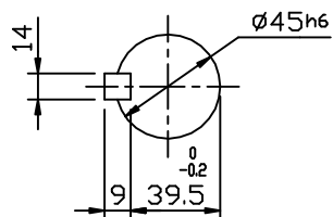
OUTPUT SHAFT
