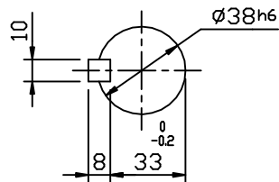
OUTPUT SHAFT
