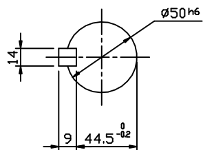
OUTPUT SHAFT
