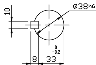
OUTPUT SHAFT
