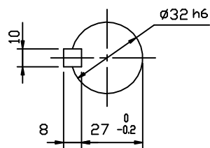
OUTPUT SHAFT
