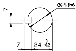
OUTPUT SHAFT
