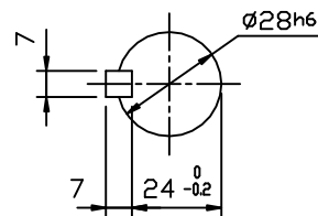
OUTPUT SHAFT
