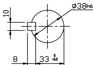
OUTPUT SHAFT
