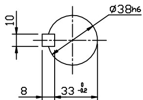
OUTPUT SHAFT
