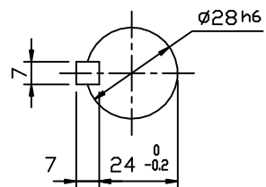
OUTPUT SHAFT
