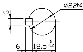
OUTPUT SHAFT
