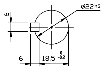
OUTPUT SHAFT
