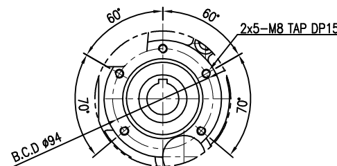
OUTPUT MOUNTING
