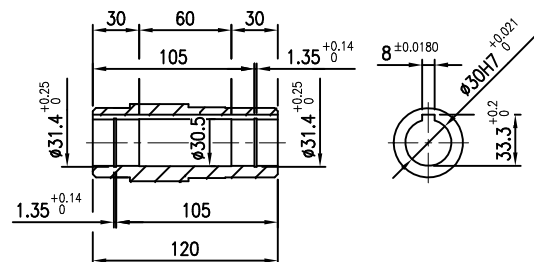
OUTPUT SHAFT(HOLLOW)
