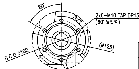
OUTPUT MOUNTING
