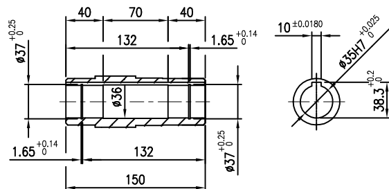
OUTPUT SHAFT(HOLLOW)
